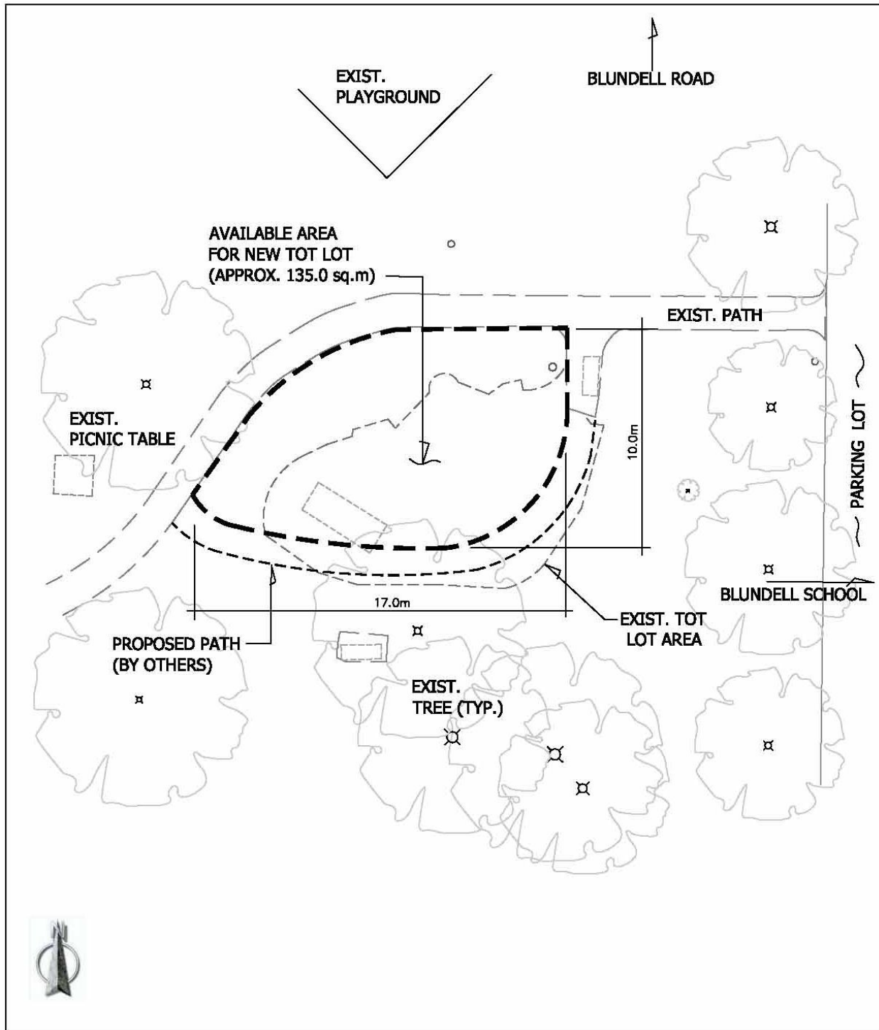
Figure 2: Blundell Preschool Playground Site Plan
